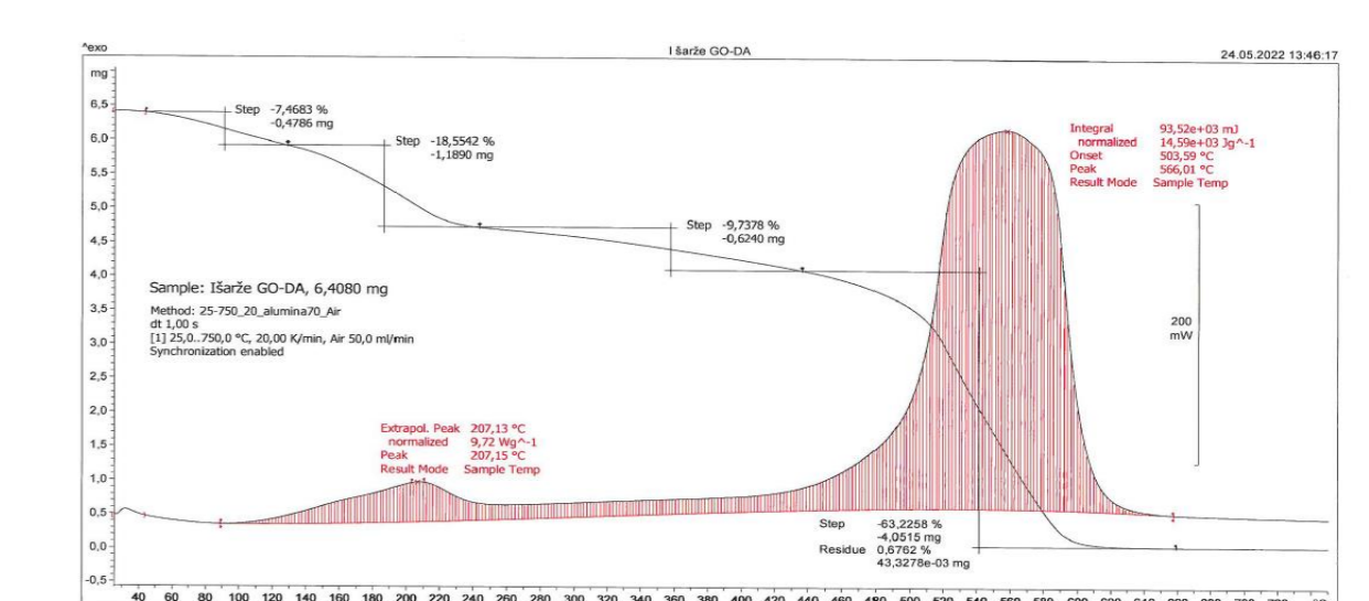
Figure 3 Thermal analysis data measured for GO-PDA (TGA/DSC curves)
