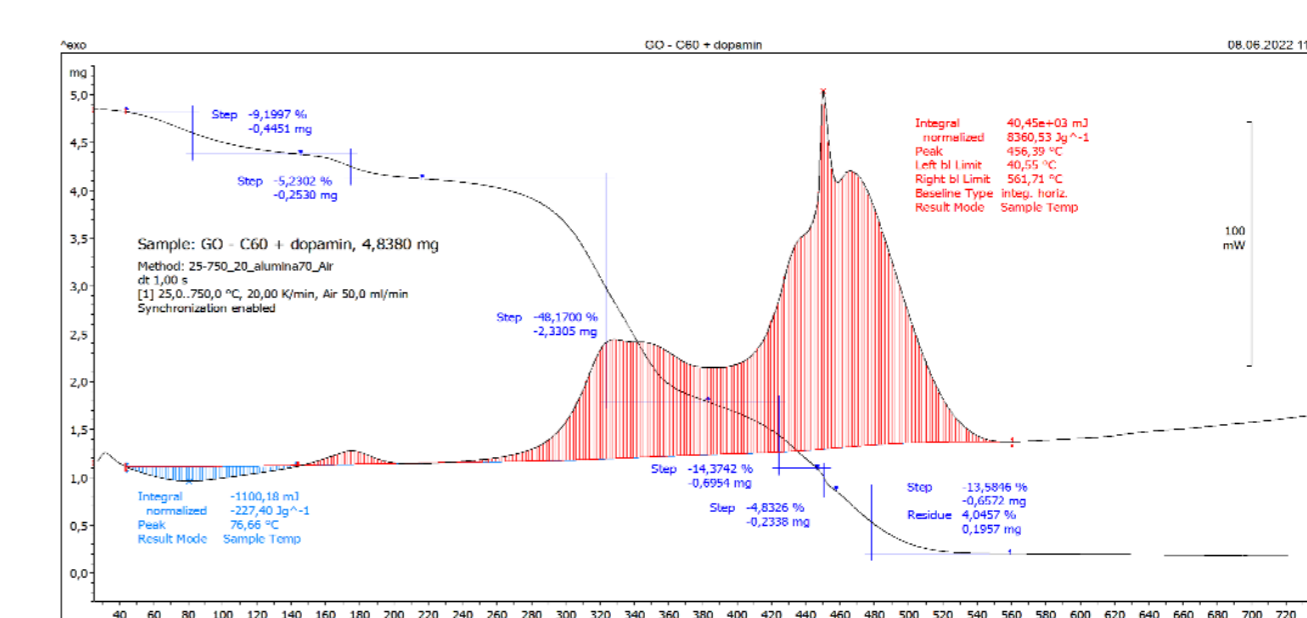
Figure 4 Thermal analysis data measured for GO-C 60 -PDA (TGA/DSC curves)
