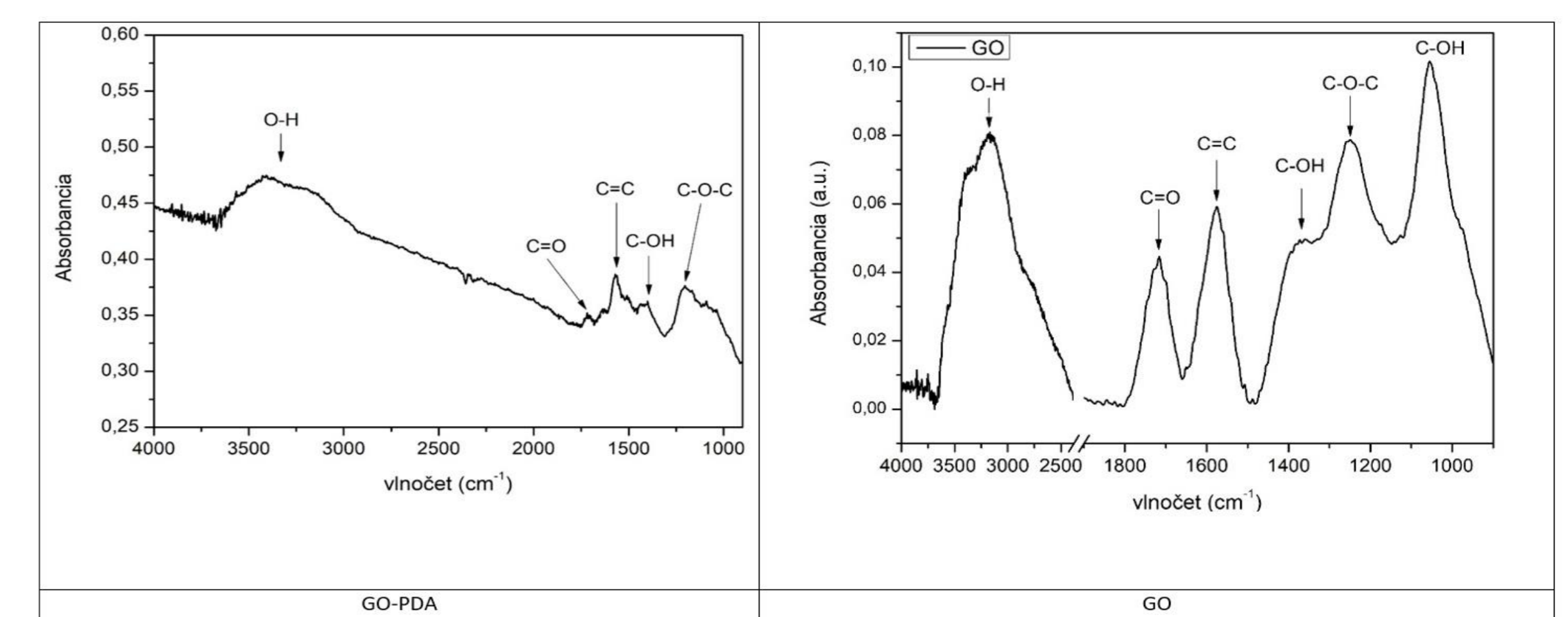
Figure 1 The FTIR spectra of GO and product formed on reaction of GO and PDA (GO-PDA)
