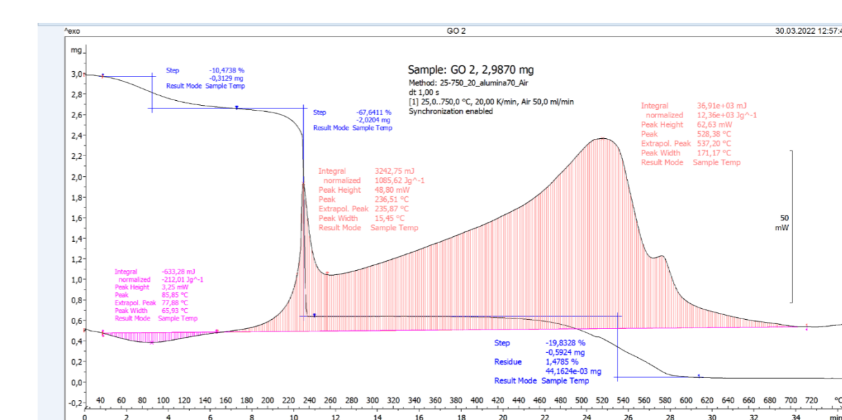
Figure 2 Thermal analysis data measured for GO (TGA/DSC curves)
